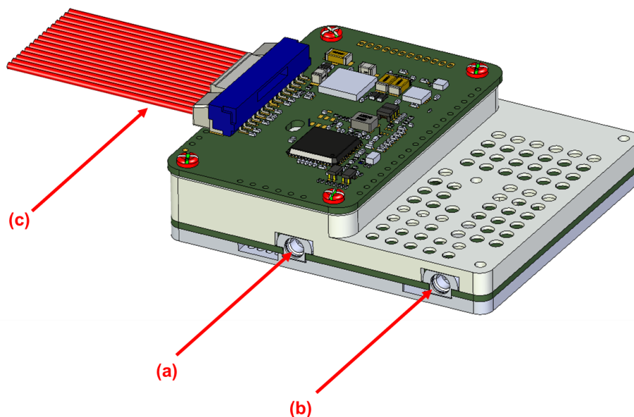
Fig. 1 Wearable Mesh Rider Radio Overview
