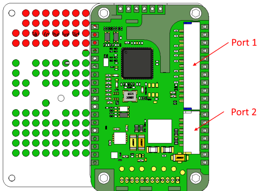
RM-5700-2L Top view
